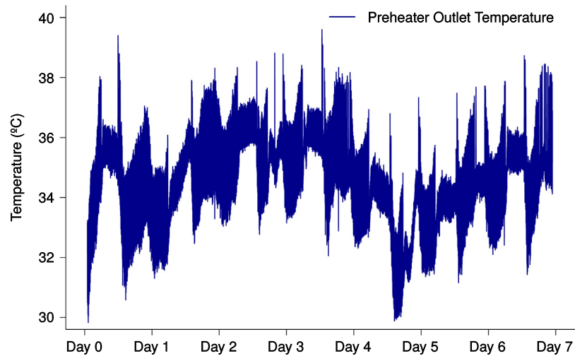
Fig. 8. Preheater outlet temperature over a seven-day period (prior to pressure reduction).
