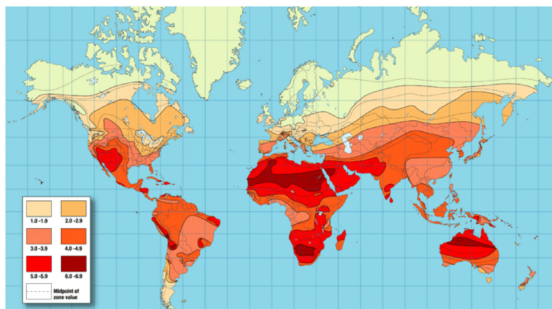
Fig. 3. Solar insolation Map of the World (Adel, 2012).
