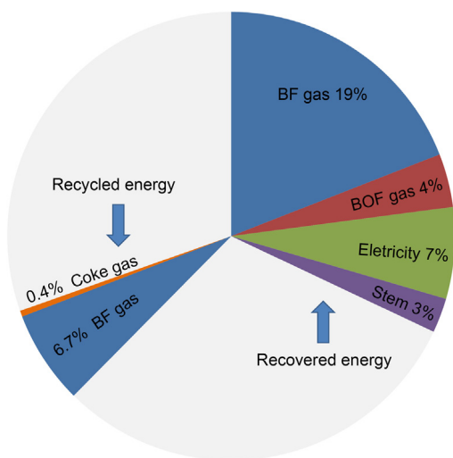
Fig. 4. The shares of recovered and recycled energy for one metric ton of crude steel.
