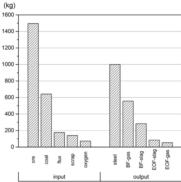
Fig. 2. Ranks of material consumption and byproducts per metric ton of crude steel.
