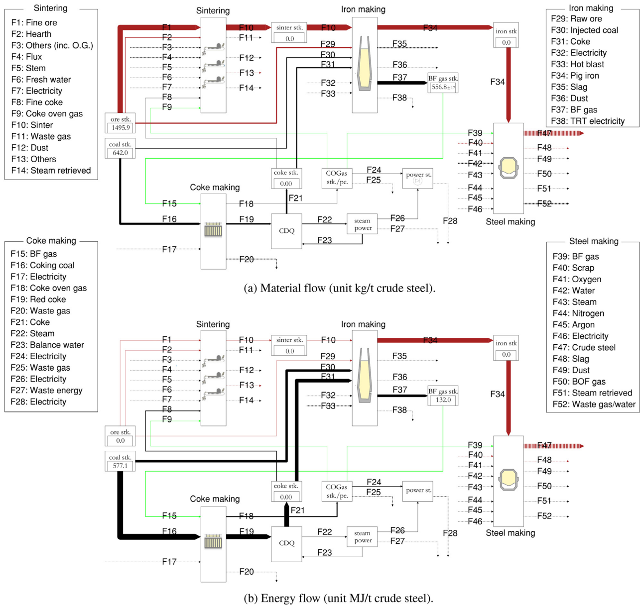
Fig. 5. Material and energy flow model for one metric ton of crude steel.
