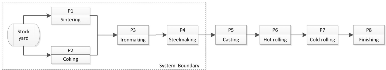
Fig. 1. The key iron and steelmaking processes and the system boundary.
