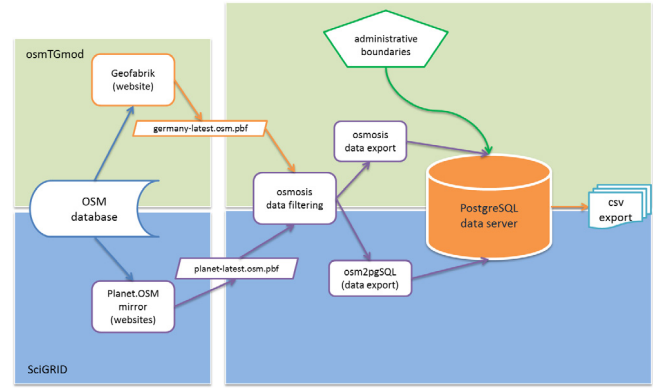
Fig. 4. SciGRID and osmTGmod work flow charts displaying the different steps and open source software involved in both models.
