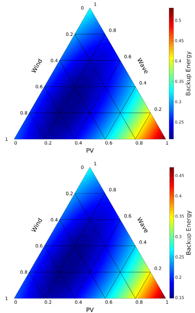
Fig. 3. Backup energy need of the isolated Iberian Peninsula in units of the consumption in dependency of the wind/PV/wave generation mix. Top: Without hydro. Bottom: With hydro.
