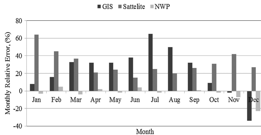
Fig. 6. Monthly relative error for Salalah station.
