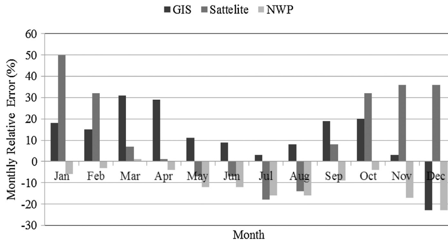
Fig. 4. Monthly relative error for Ibrri station.
