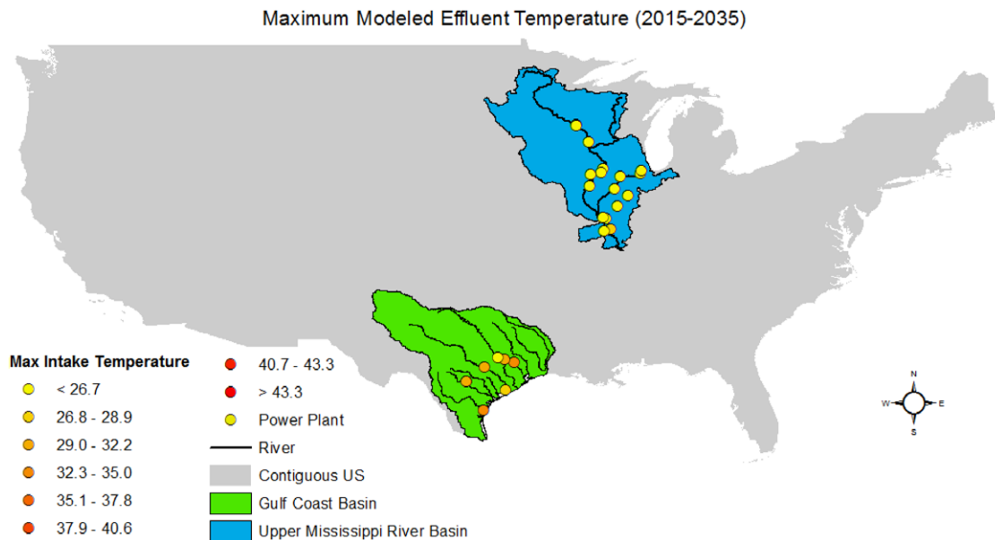
Fig. 7. Intake temperature is important for cooling efficiency and safety of equipment. Moreover, intake temperature approaching effluent temperature limits increase a power plant's risk of exceeding the limit and reduce cooling capability per unit of water. Six plants modeled in this analysis could face intake temperatures in excess of 28.9 °C between 2015 and 2035.
