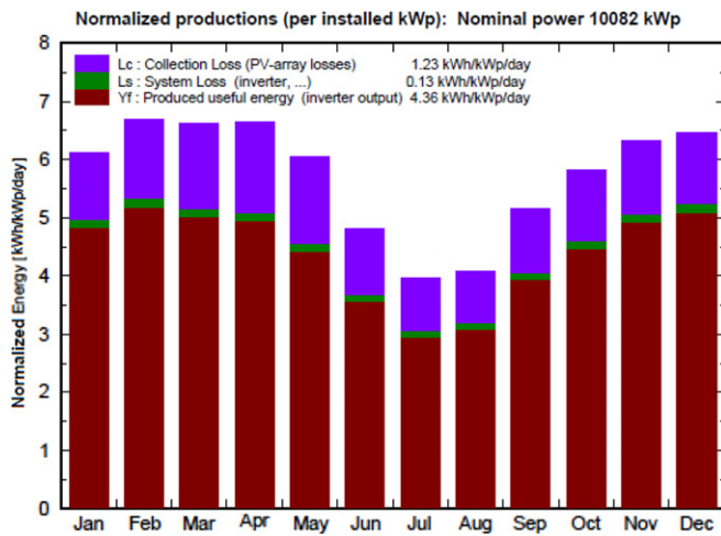
Fig. 6. Normalized energy per month.
