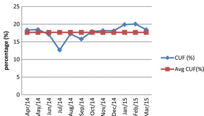
Fig. 5. Average capacity utilization factor in various month.
