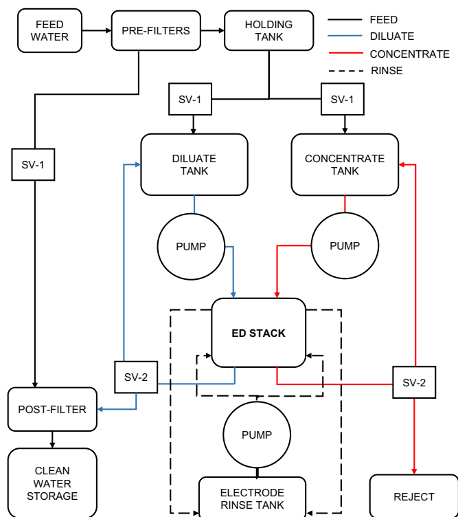
Fig. 9. Flow path of an in-home ED water treatment system including pre- and post-filtration components.
