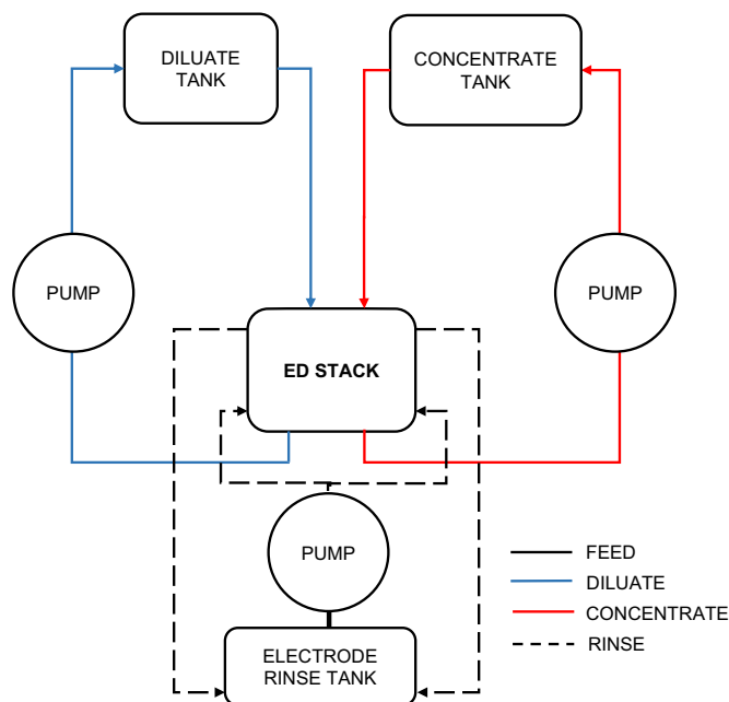
Fig. 7. Flow diagram of experimental setup.
