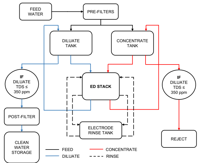
Fig. 2. Flow diagram for batch ED process.
