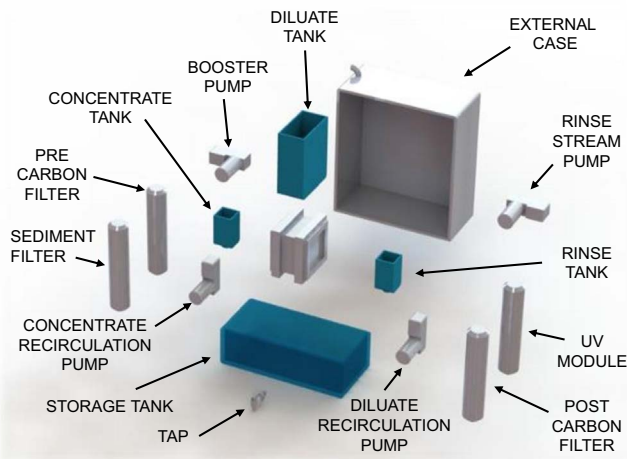
Fig. 11. Exploded view of product concept.
