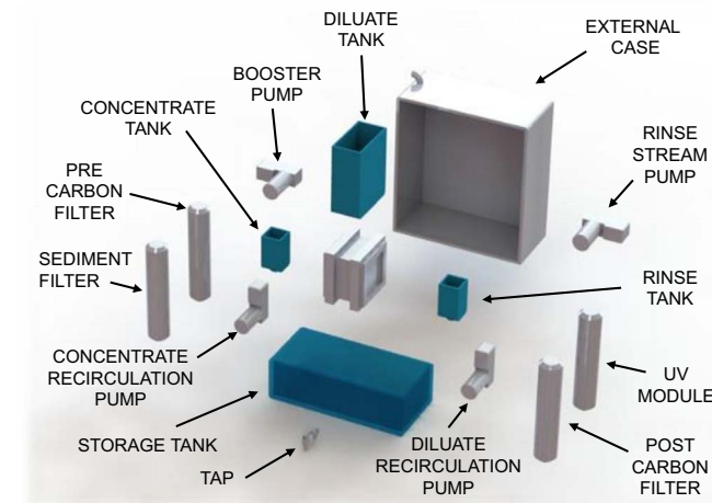
Fig. 11. Exploded view of product concept.
