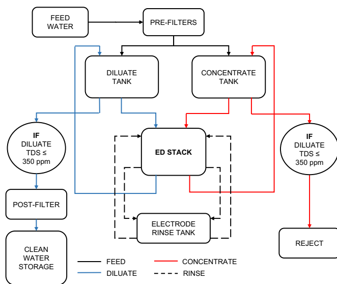
Fig. 2. Flow diagram for batch ED process.
