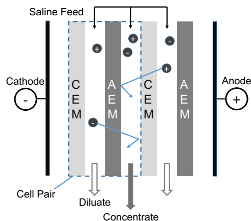
Fig. 1. A voltage potential is applied across a series of alternating cathode exchange membranes (CEM) and anion exchange membranes (AEM) in an Electrodeposition (ED) stack to separate the feed solution to concentrate and diluate streams.
