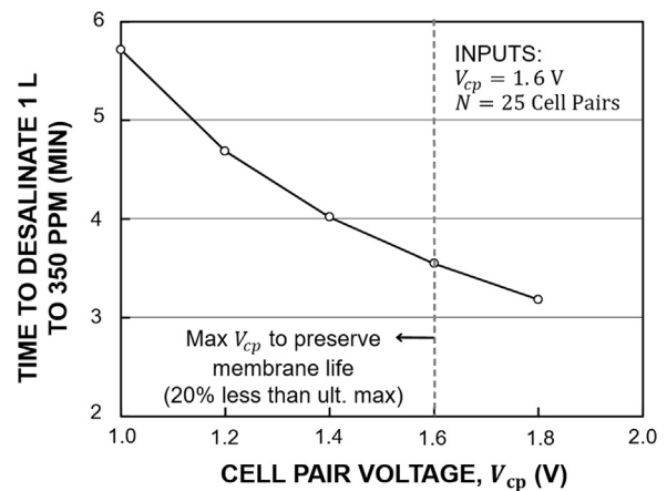
Fig. 5. Model results showing time to desalinate 1 L of diluate from 3000 ppm to 350 ppm for varying cell pair voltages across 25 cell pairs.
