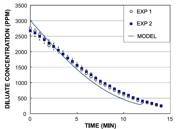
Fig. 8. Diluate concentration plotted against time for two identical tests (EXP 1 and EXP 2) using 18 cell pairs, 1.6 V/cell pair, and at a circulation rate of 72 L/h. Error bars represent Type B uncertainty of 6–8% in concentration measurements.
