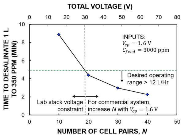
Fig. 6. Model results showing time to desalinate 1 L of diluate from 3000 ppm to 350 ppm for increasing number of cell pairs, each producing a voltage drop of 1.6 V. The horizontal and vertical dashed lines indicate the desired operating range and test stack constraints respectively.
