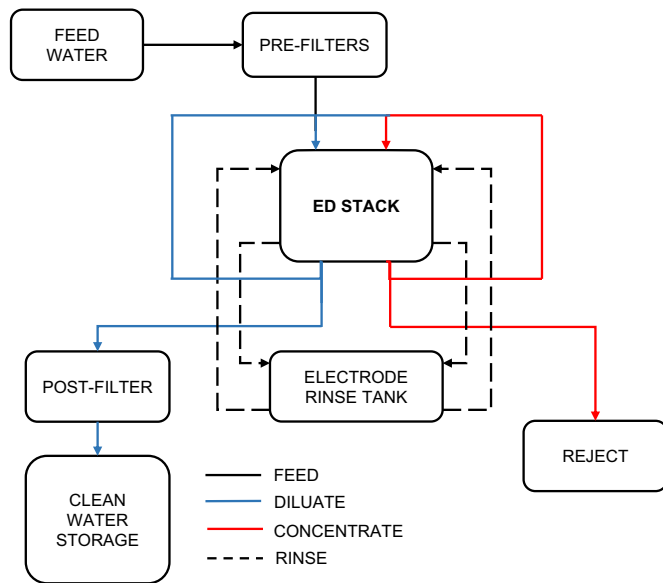
Fig. 3. Flow diagram for continuous ED process.
