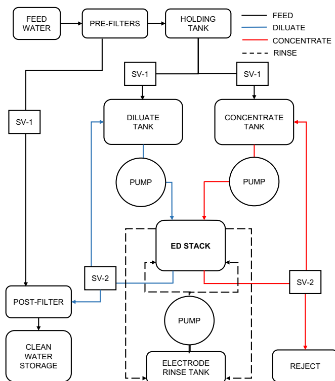
Fig. 9. Flow path of an in-home ED water treatment system including pre- and post-filtration components.
