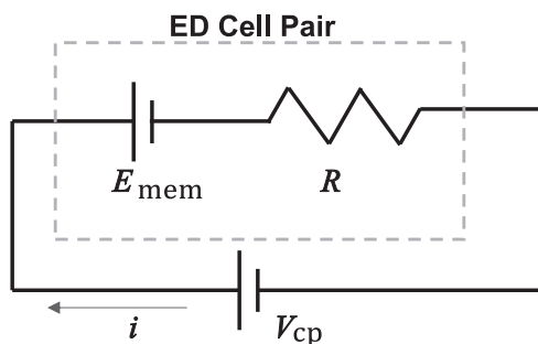
Fig. 4. Simplified depiction of an ED cell pair using an electrical circuit analogue.
