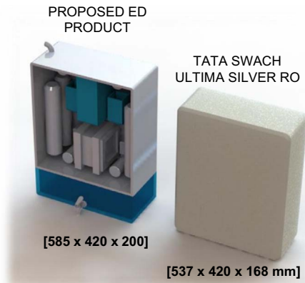
Fig. 10. Comparison of product dimensions between the ED concept and the Tata Swach Ultima Silver RO unit (Tata Chemicals Ltd, 2014).
