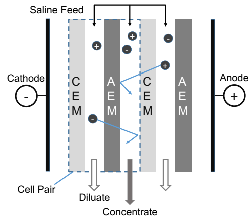
Fig. 1. A voltage potential is applied across a series of alternating cathode exchange membranes (CEM) and anion exchange membranes (AEM) in an Electrodialysis (ED) stack to separate the feed solution to concentrate and diluate streams.
