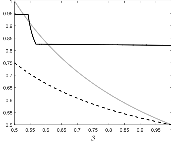
Figure A.1: t^a(\beta) (in gray), \mathbf{E}[\theta | \theta > t^h(\beta)] (in black) and t^h(\beta) (dashed) as functions of \beta for \theta distributed as in (A.7).
