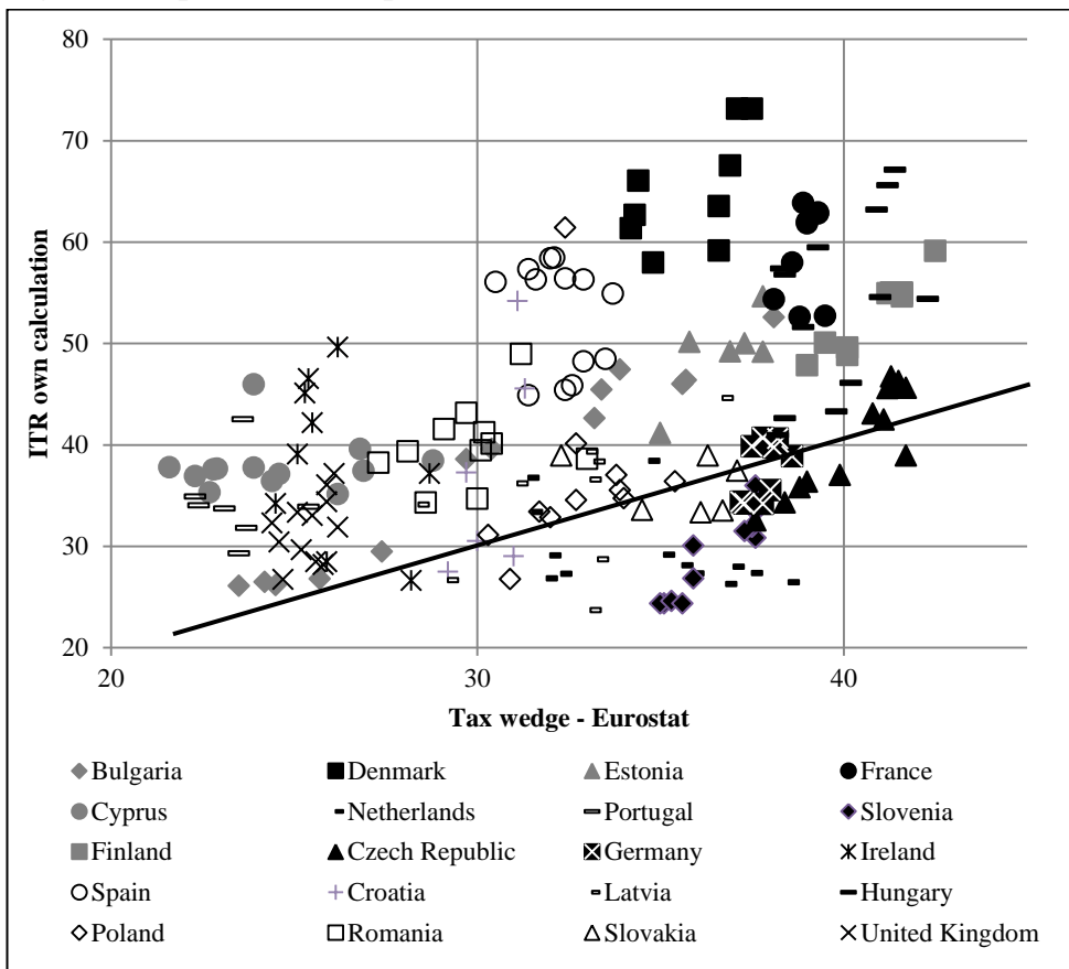
Fig. 3 Comparison of computed data and Eurostat data
