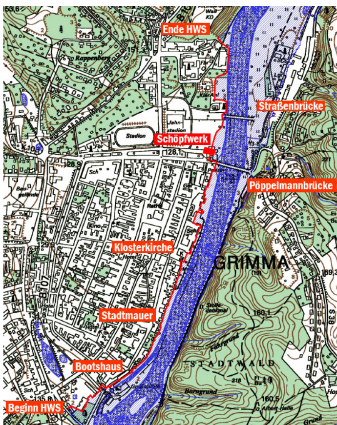
Figure 25 Flood wall projects for the town of Grimma (hochwasserschutz-grimma.de, 2017)
