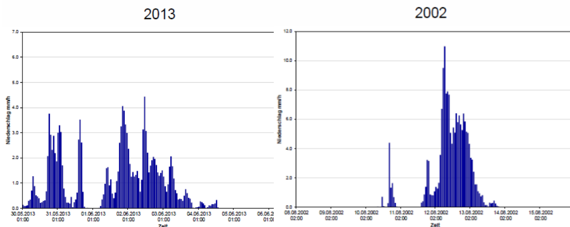
Figure 9 Rainfall intensity [mm/h] in time for the 2013 and 2002 flood events in Pegel Bad Dübren 1/Vereinigte Mulde gaging station (Schumann et al., 2016)
