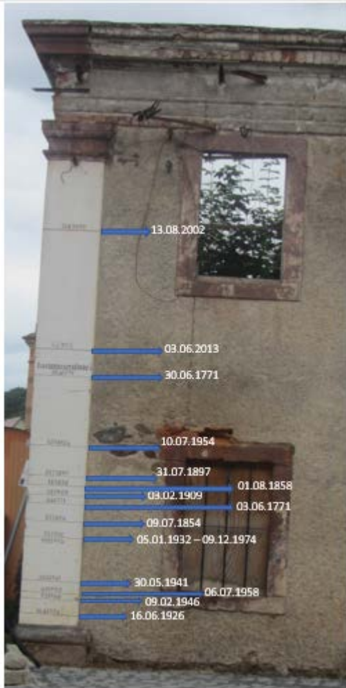
Figure 15 Historic flood levels in the Großmühle (large mill) in Grimma (2017, author).
