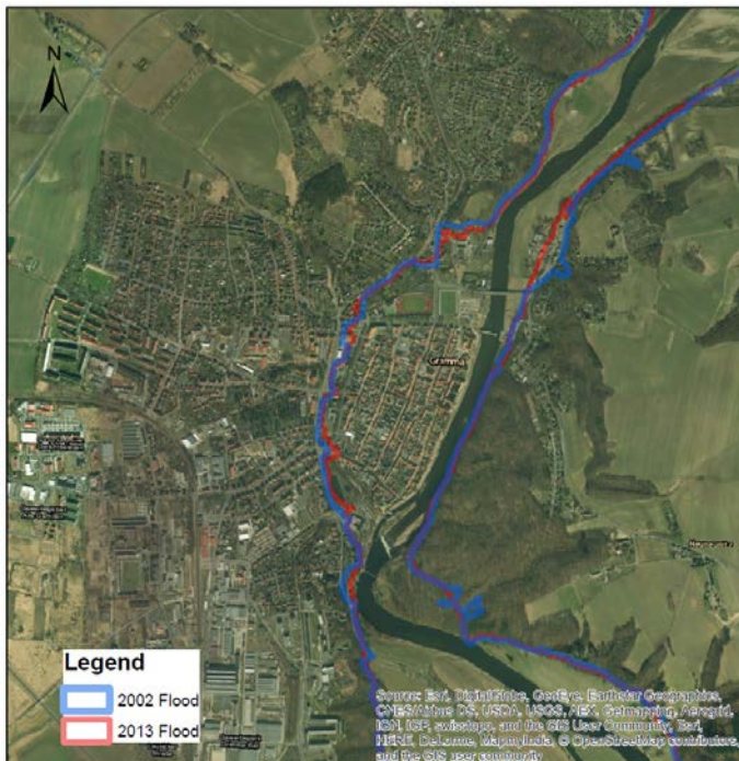
Figure 13 Map of the flooded areas in 2002 and 2013 (elaborated with data from the Saxony State Office for Environment, Agriculture and Geology, 2017).
