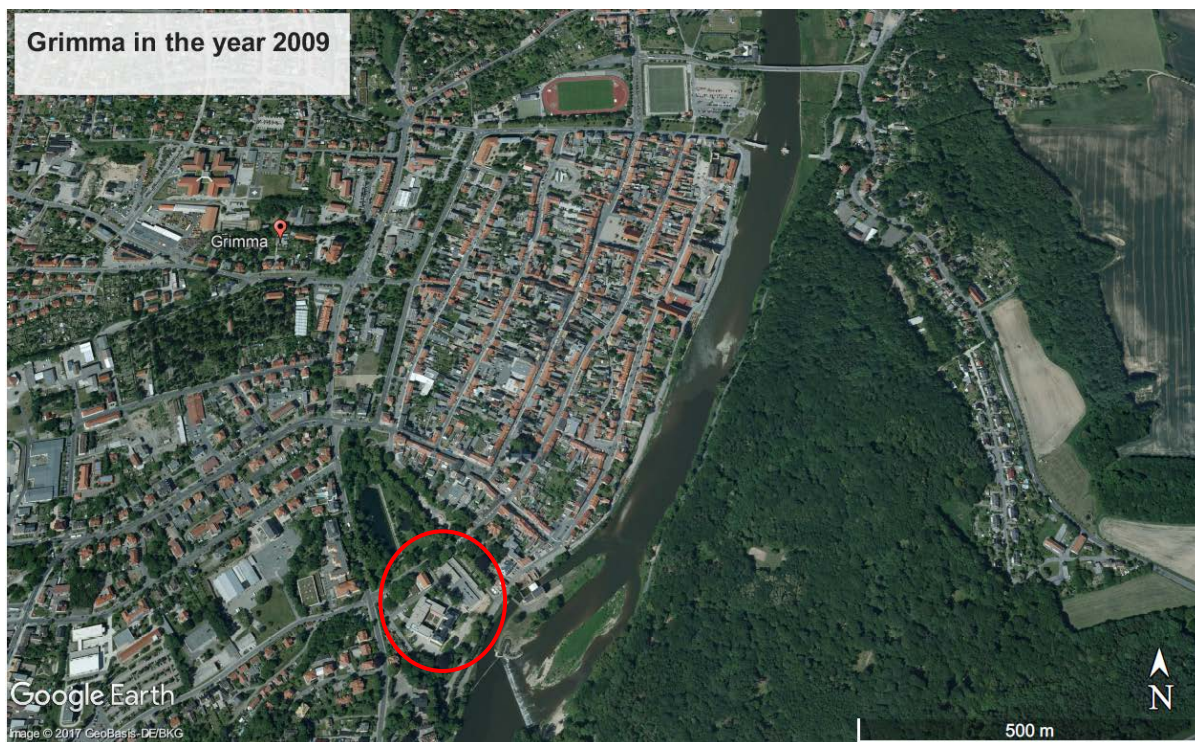
Figure 21 Satellite image of Grimma in 31-12-2009 (Google Earth2017)
