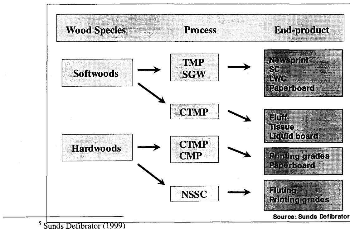
Figure 3. Selection of mechanical pulping process by raw material and end-product
