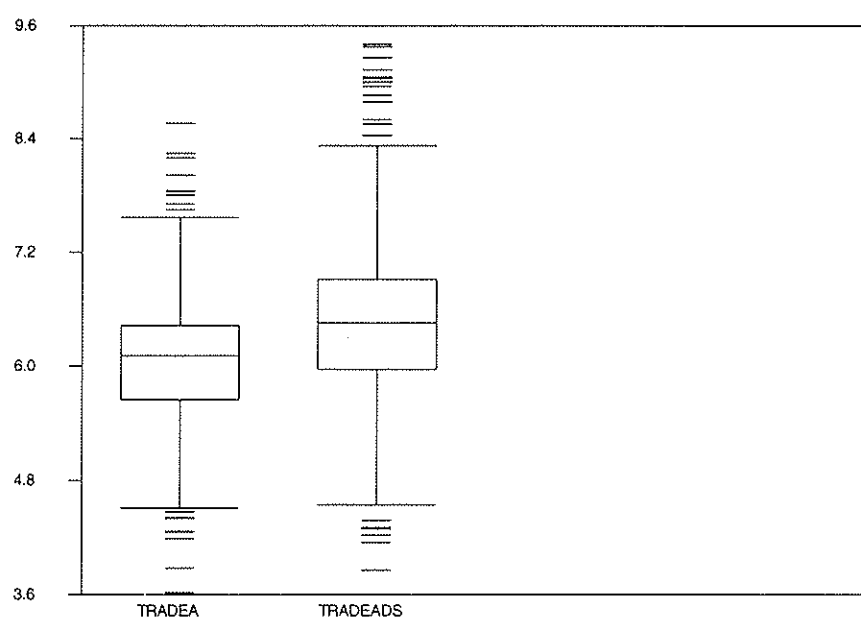
Figure 2. Box-plot. Trading volume of Nokia A and ADS (in logs).
