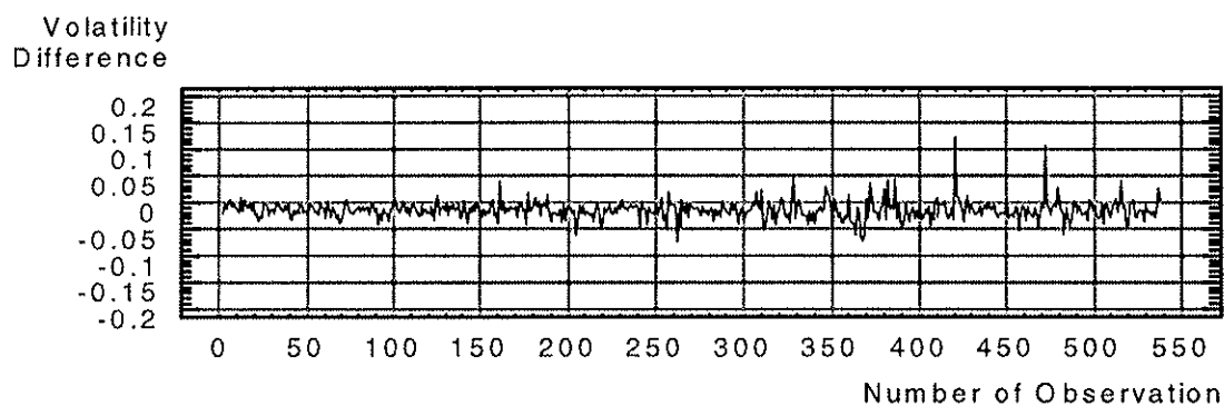
Figure 5. Time sequence plot. Volatility difference between Nokia A and ADS.
