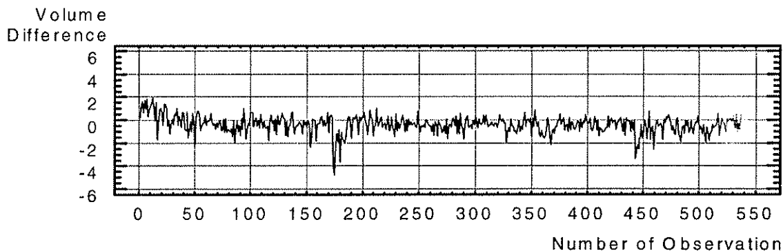
Figure 6. Time sequence plot. Volume difference between Nokia A and ADS.
