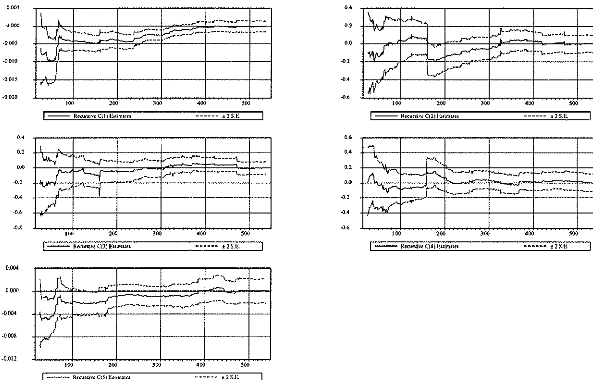
Figure 6. Recursively estimated parameters from the model (34). Lower and upper lines respond \pm 2 *standard error. C(i) denote i^{\text{th}} estimator of the estimated model.
