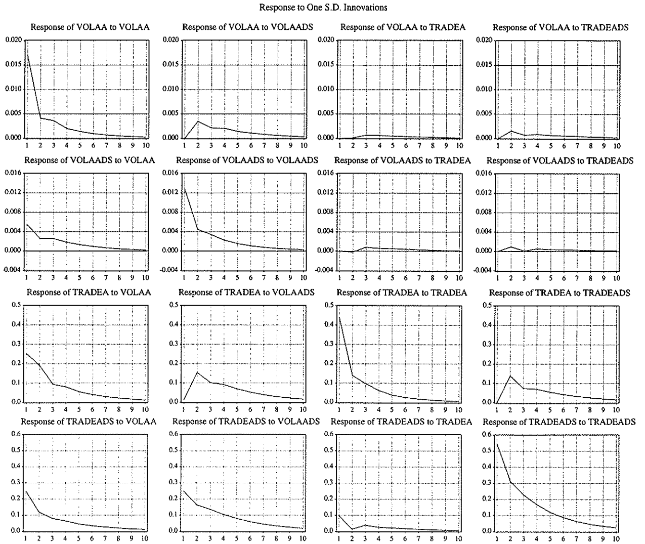
Figure 7. Impulse Response Functions. Number of days after shock in horizontal axis, in vertical axis the variable which responds to 1 standard deviation shock of the other variable.
