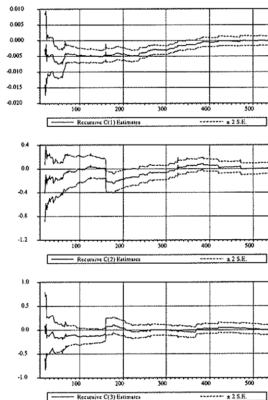
Figure 3. Recursively estimated parameters from the model (33). Lower and upper lines respond \pm 2 *standard error. C(i) denote i^{\text{th}} estimator of the estimated model.
