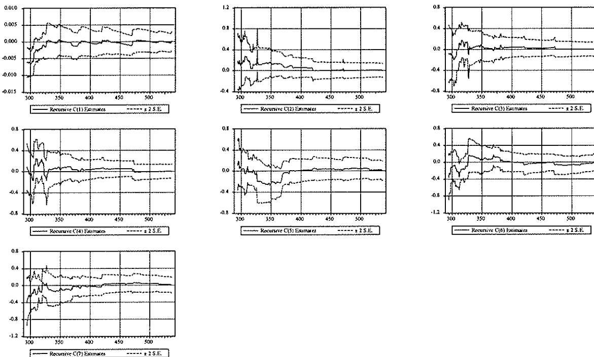
Figure 5. Recursively estimated parameters from the model (33). Lower and upper lines respond \pm 2 *standard error. C(i) denote i^{\text{th}} estimator of the estimated model.
