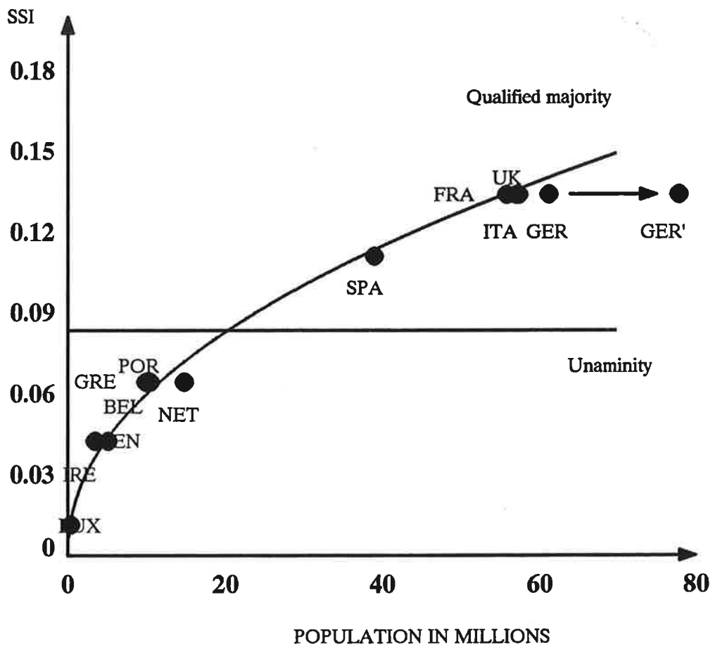
Figure1. SSI and population in the EC12
