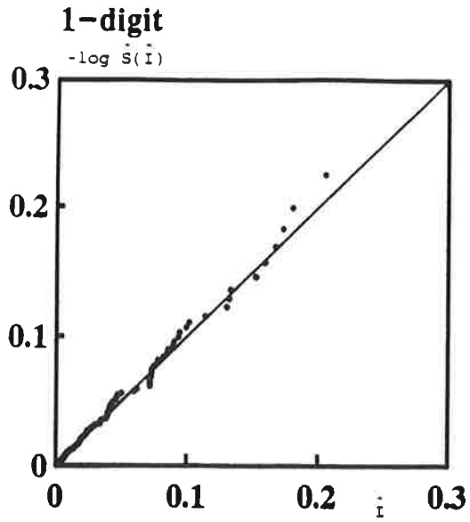
Fig. 1. Residual plots of Gompertz models
