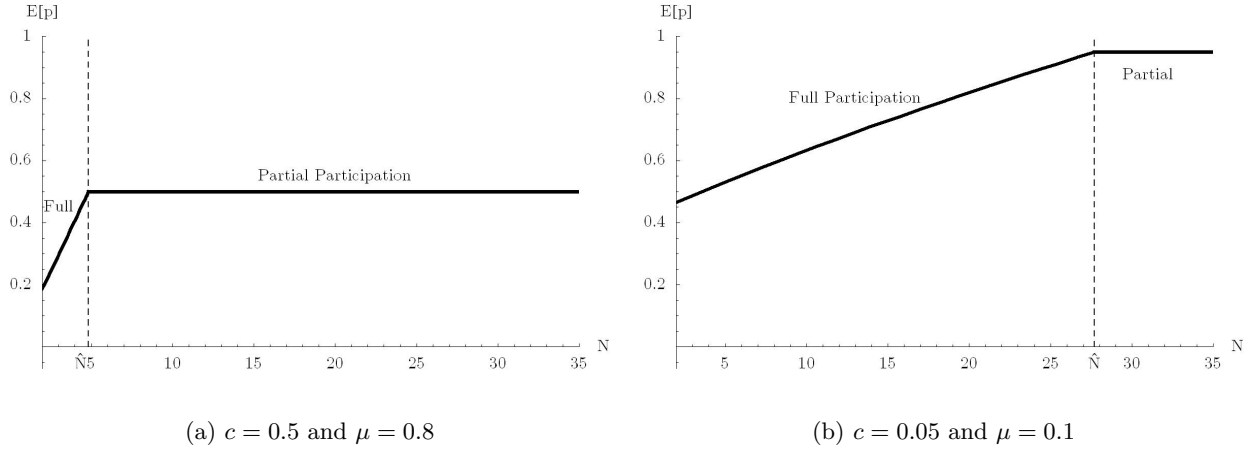
Figure 5: The impact of N on expected price
