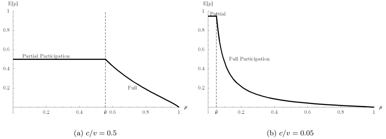
Figure 3: The influence of \mu on expected price ( N = 2 ).
