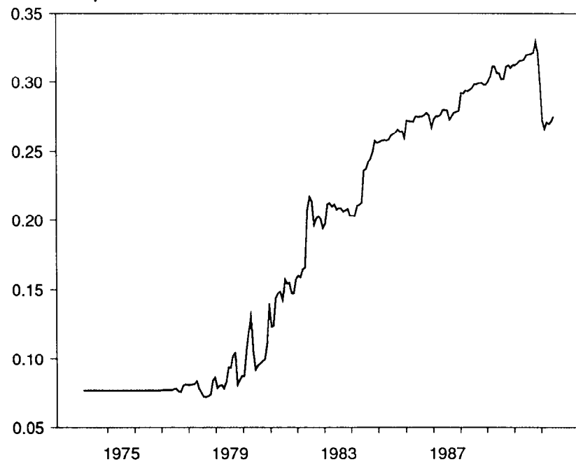
A. Coefficient for Default Risk
