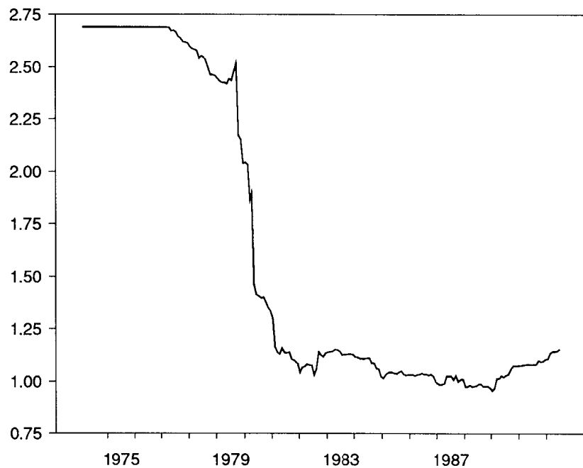
C. Coefficient for the Federal Funds Rate
