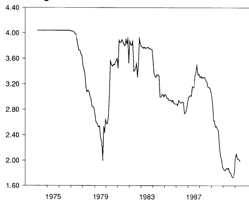
B. Coefficient for Inventories
