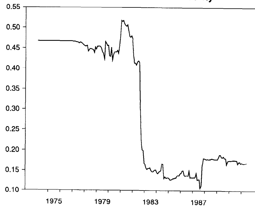
D. Coefficient for Stock Return Volatility
