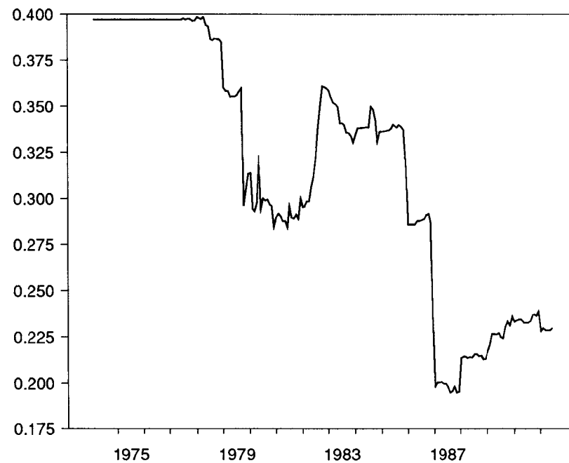
D. Coefficient for Federal Funds Rate Volatility
