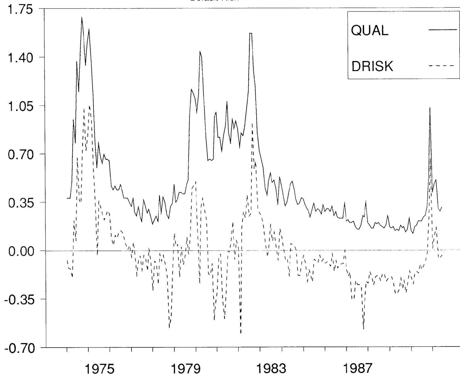
Figure 2 Default Risk
