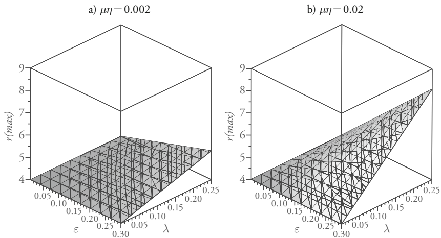
Figure 1: Threshold Value of Real Interest Rate
