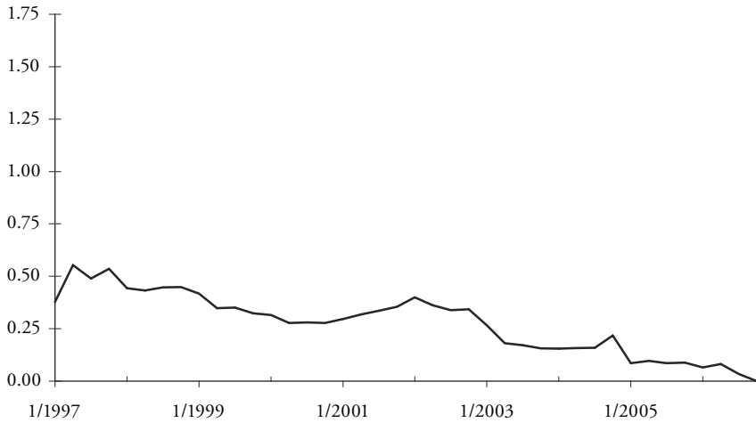
Figure 6: Cointegrating Relations
