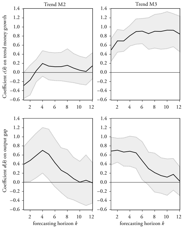
Figure 6: Coefficients on Trend Money Growth and the Output Gap in Equation (4)
