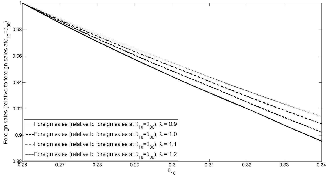
Figure C.3b: Sales, \bar{z} = 1.5, c_1 = 0.85c_0
