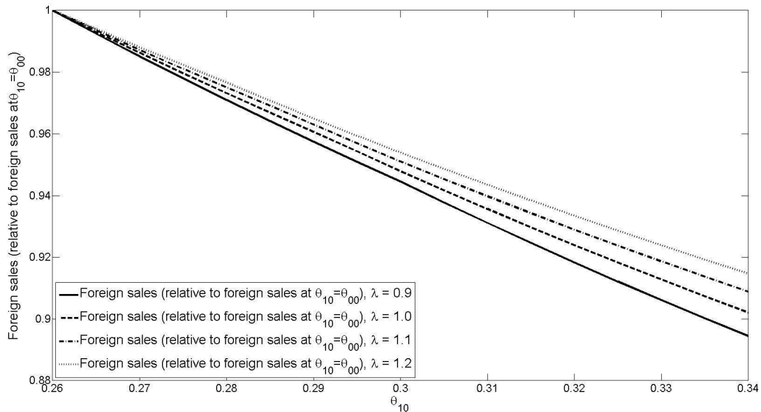
Figure C.4b: Sales, \bar{z} = 3, c_1 = 0.85c_0
