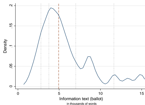
FIGURE A.1. VARIATION IN THE BOOKLET-BASED COMPLEXITY MEASURE
