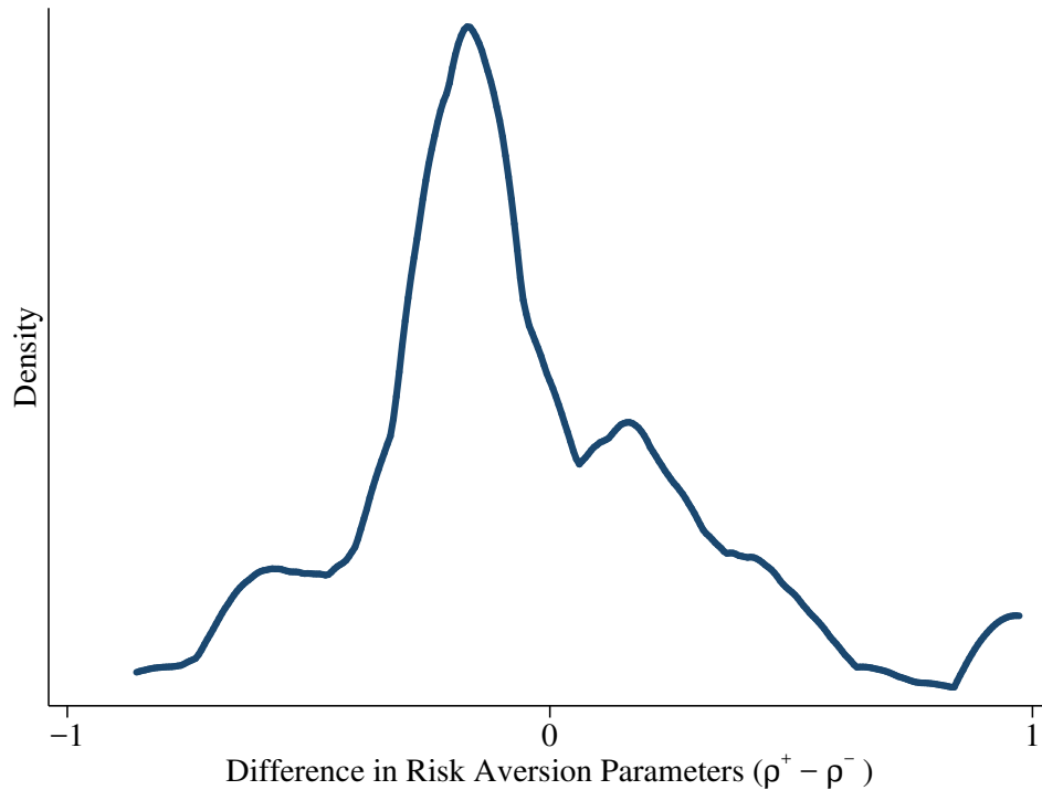
Figure F.1: On average the risk aversion parameter is similar in the loss and gain domains.
