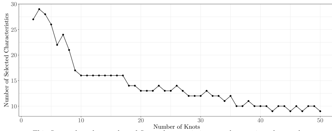
Figure 6: Number of Selected Characteristics versus Number of Interpolation Points
