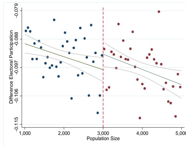
Figure 2: LLR estimates
