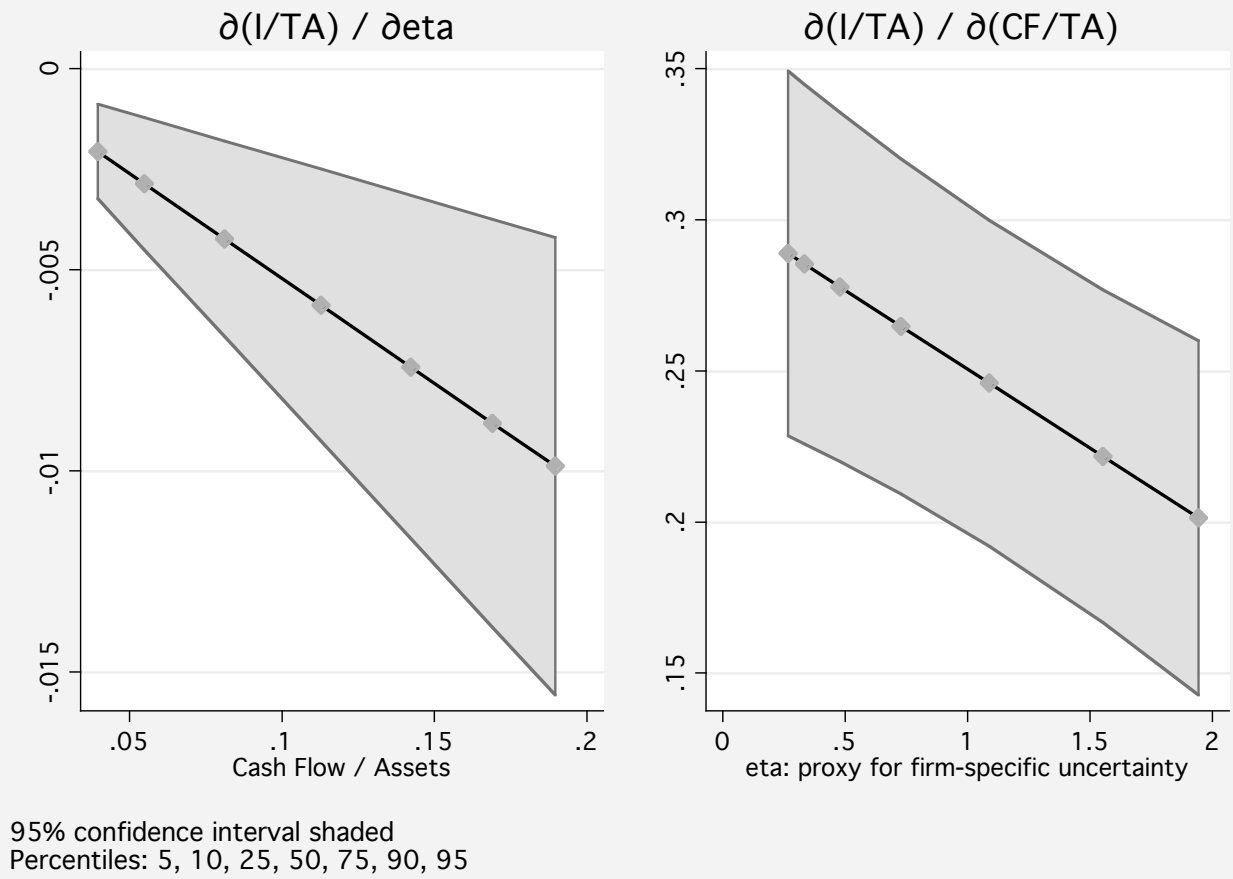
Figure 1. Estimated sensitivities from interactions model
