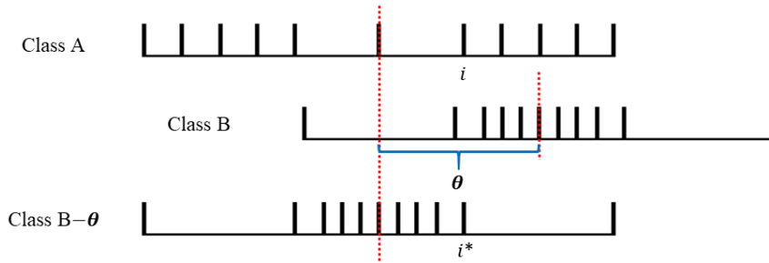
B: Test Scores distributions in schools with same mean, min and max
