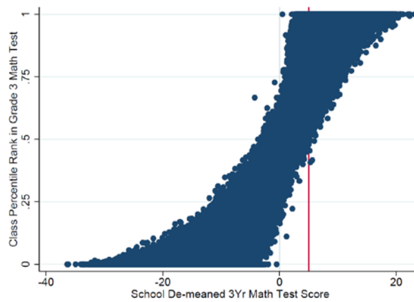
C: Variation in class rank conditional on test scores
