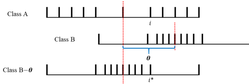
B: Test Scores distributions in schools with same mean, min and max
