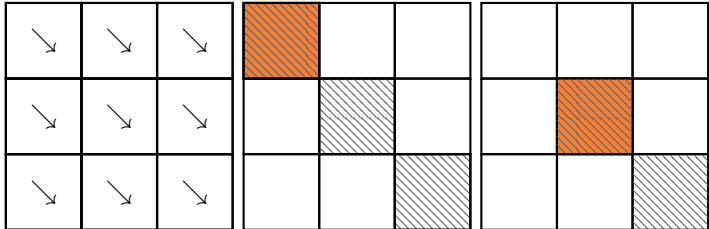
Figure 1: Illustrating public good source and exposure in the presence of spillovers
