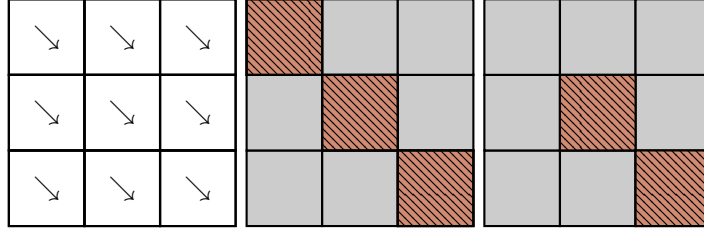
Figure 3: Illustrating the average exposure effect estimator
