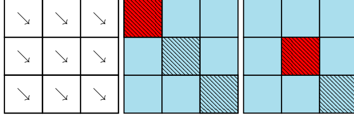
Figure 2: Illustrating the average source effect estimator
