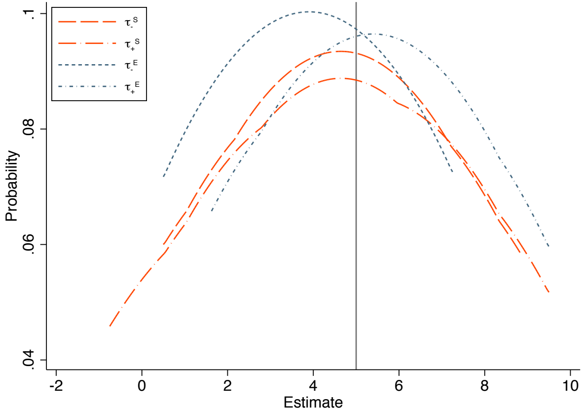
Figure 4: Distribution of estimates of ASEE and AEEE for different configuration of baseline characteristics
