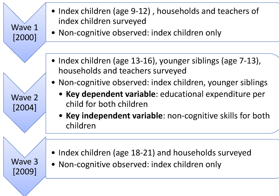
Figure 1: Data structure
