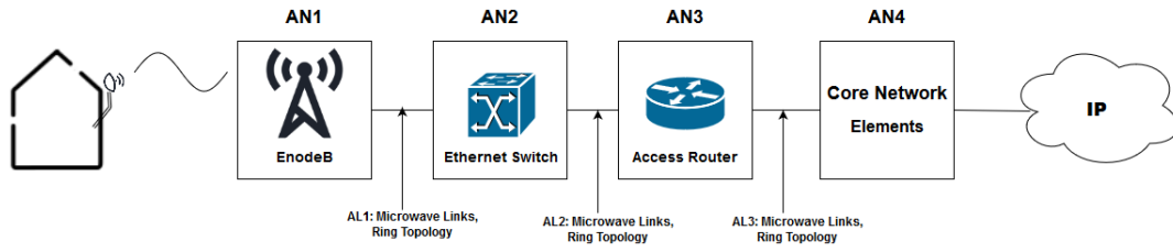
Fig 1. LTE FWA network architecture
