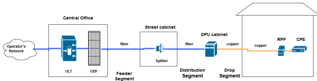
Fig 2. G.fast FTTdp street network architecture
