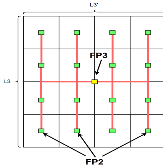
Fig 4. Example of Geometric model for FP3 (Layer 3).
