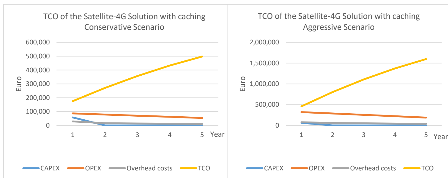
Figure 5 Total expenditures of satellite-4G solution with caching data on the edge
