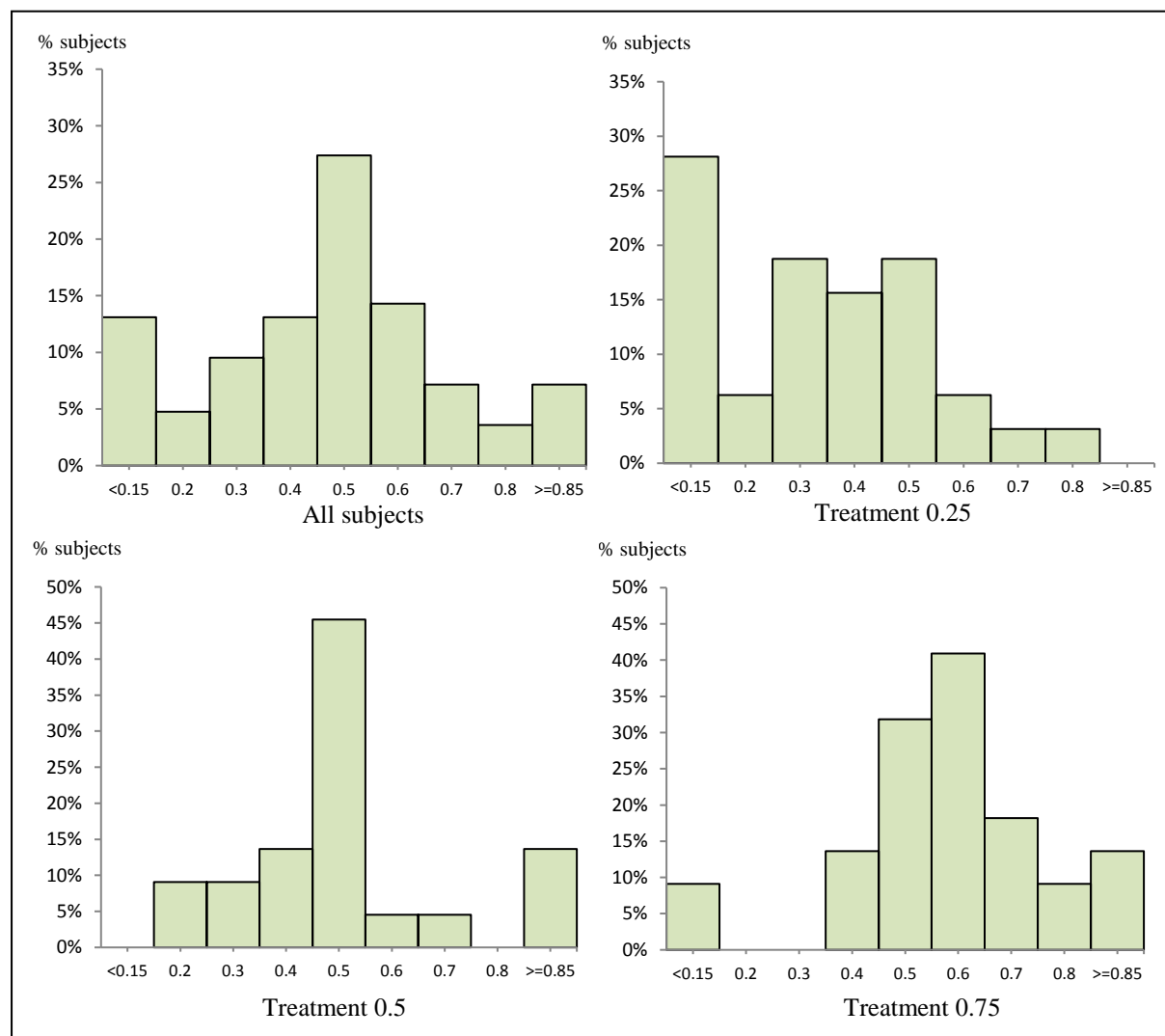
Figure 1: Revealed Belief
