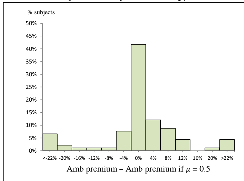
Figure 3: The impact of estimating \mu
