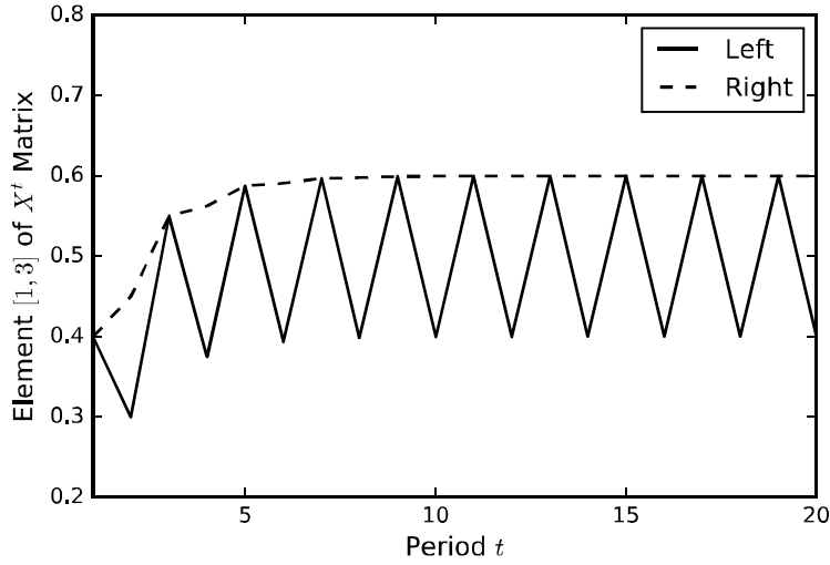
Figure 1: Convergence in Markov Chain and Cultural Transmission Models – Counterexample tic matrices depends on whether multiplication is from the right as in Markov chain models or the left as in the cultural traits transmission literature discussed here. Furthermore, for left multiplication, the example is a simple sequence of matrices that does not converge in a cultural transmission context. Both points play an important role in the inaccuracies in the convergence proof of P14 that we describe below.
