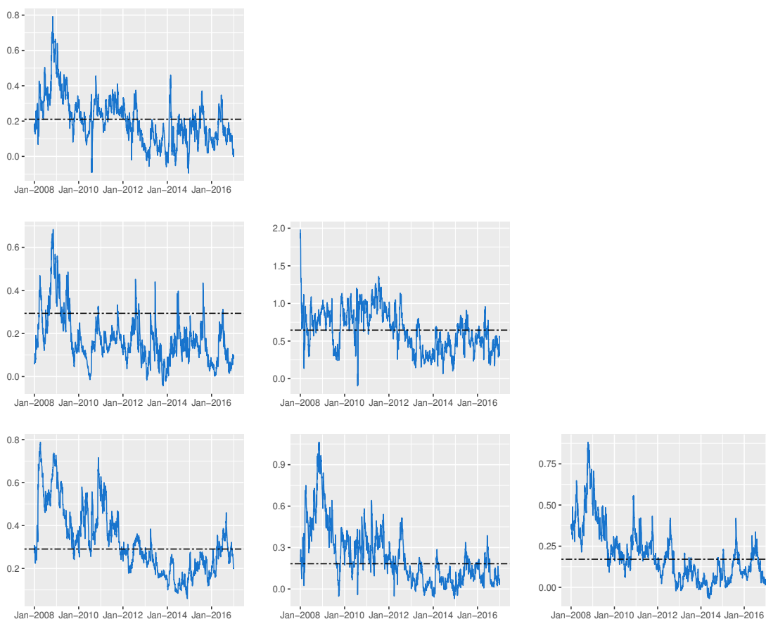
Figure 4: Optimal dynamic hedge ratios corresponding to \begin{pmatrix} hr_{21,t} & & \\ hr_{31,t} & hr_{32,t} & \\ hr_{14,t} & hr_{24,t} & hr_{34,t} \end{pmatrix} , where 1 = sugar, 2 = wheat, 3 = soybeans, 4 = coffee.
