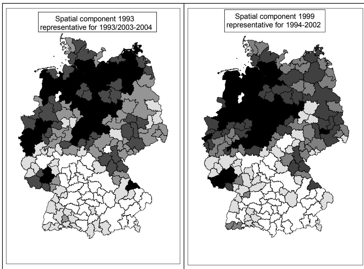
Figure 2: Map patterns of spatial components
