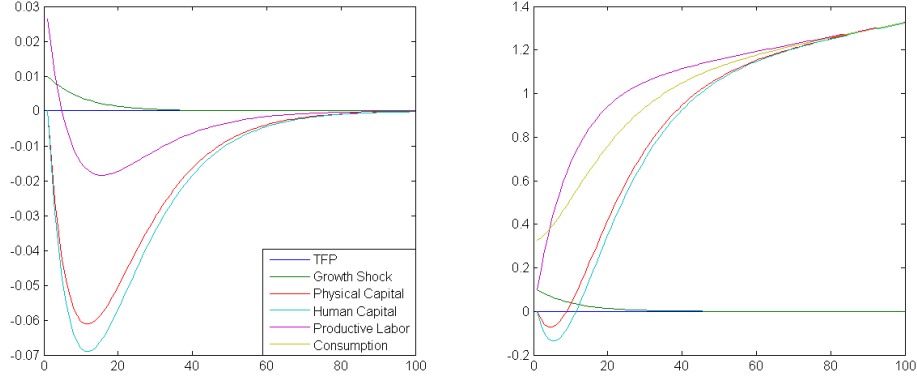
Figure 1: Impulse response functions for de-trended stationary variables (left hand panel) log levels (right hand panel)
