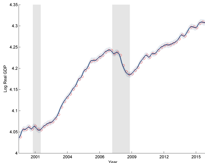
Figure 2: Estimates for monthly log real GDP at an annual rate with two standard deviation confidence intervals (estimated from the filter and smoother as opposed to simulation) over the financial crisis. Realizations for quarterly GDP are marked by circles.
