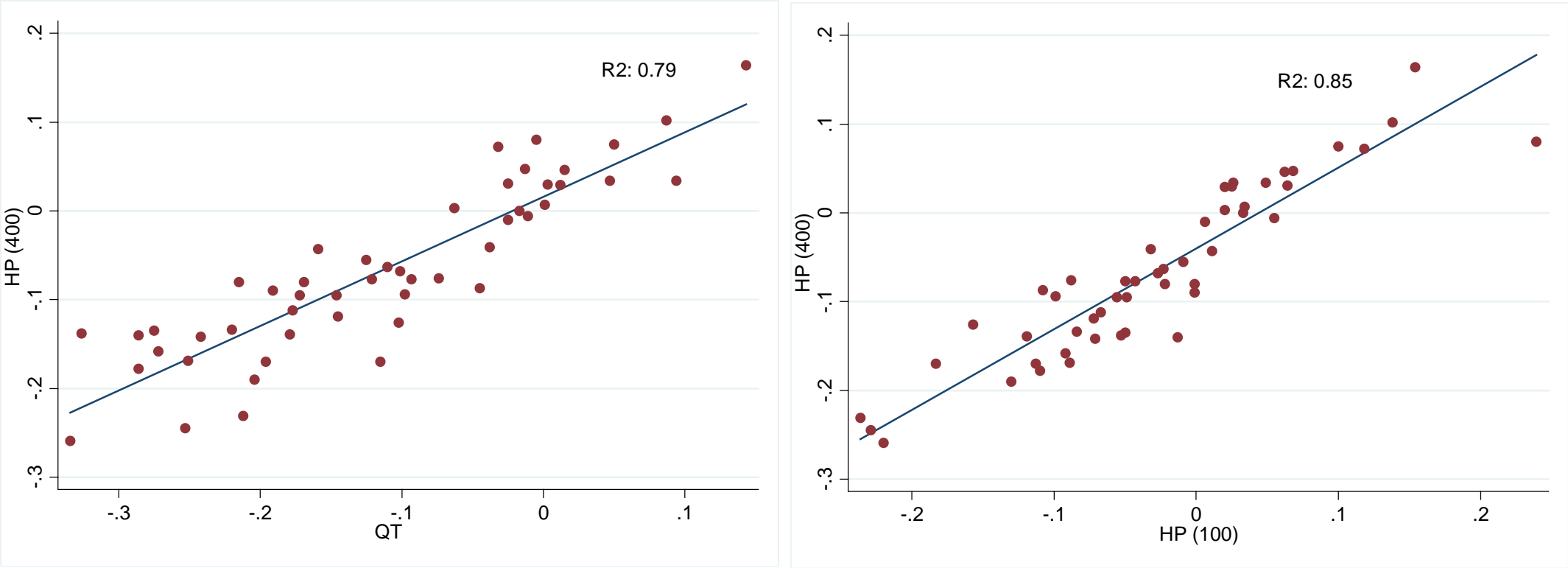
Figure A1. Scatterplot diagrams of the relationship between the cyclical sensitivities obtained by the HP method ( \lambda=400 ), HP method ( \lambda=100 ) and the QT procedure.
