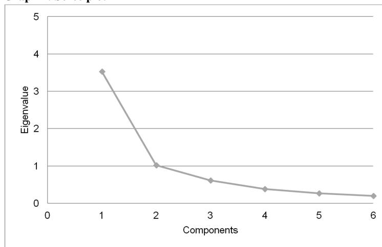
Graph 2: Scree plot
