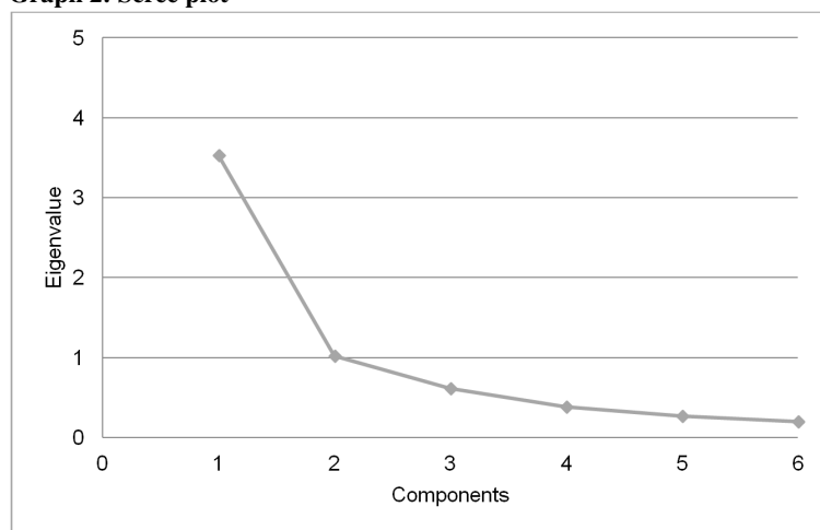
Graph 2: Scree plot
