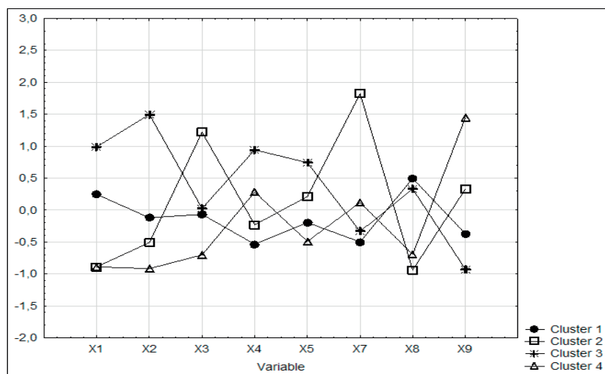
Figure 3. Means for each cluster (k=4)
