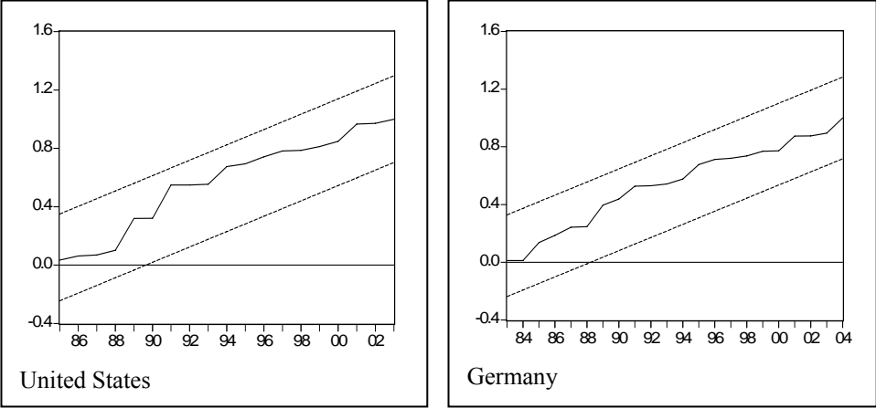
Stability Analysis for model (2): CUSUM of squares and 5% significance bounds
