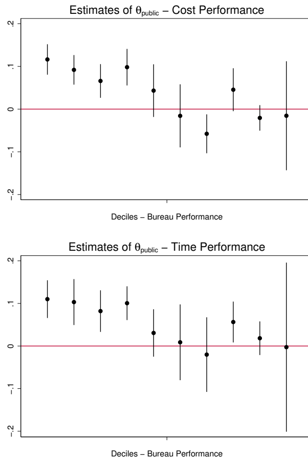
Figure 6: \hat{\theta}_{public} on deciles of bureau performance
