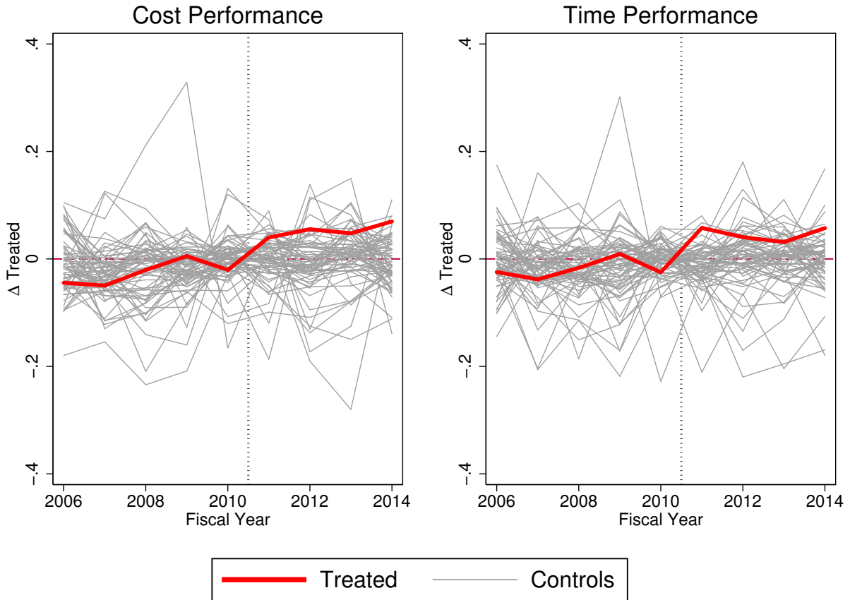
Figure 4: Synthetic Control Group - Inferential analysis
