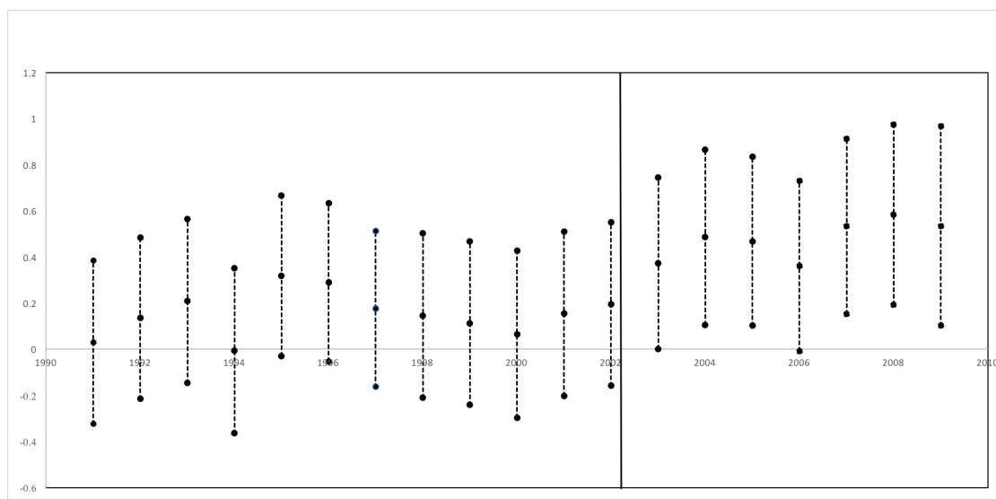
Figure 1: Falsification Exercise
