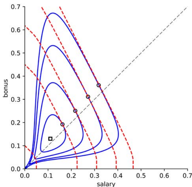
Figure 6: Iso-profit curves and iso-utility curves in contract space.
