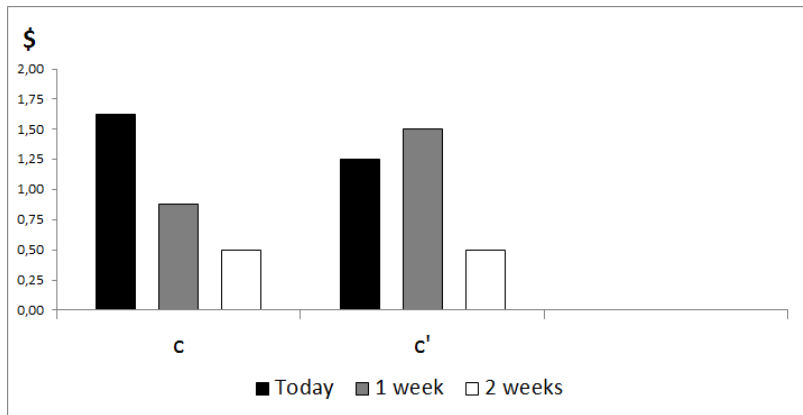
Figure 1: Decision task
