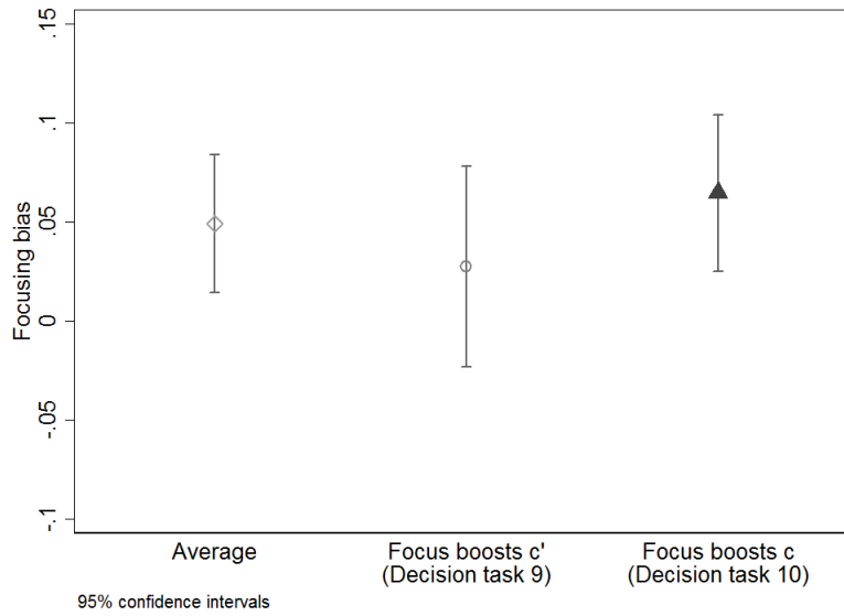
Figure 4: Focusing bias
