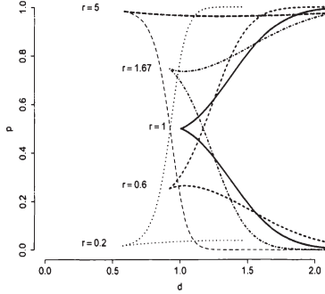
Figure 1.1: Regions of bimodality of the normal distribution, where d = (\mu_2 - \mu_1)/(2\sqrt{\sigma_1\sigma_2}) and r = \sigma_1/\sigma_2 . On the right side of the curves are those parameter constellations of p and d for which for fixed r the resulting mixture is bimodal.
