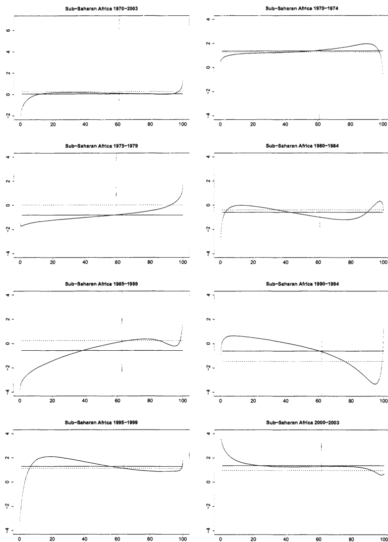
Figure C.12: Semi-decade specific Growth Incidence Curves, Sub-Saharan Africa. Solid line: Growth Incidence Curve, solid vertical line: $2 per day poverty line, solid horizontal line: mean of growth rates, dashed line: growth rate of mean, dotted line: rate of pro-poor growth.
