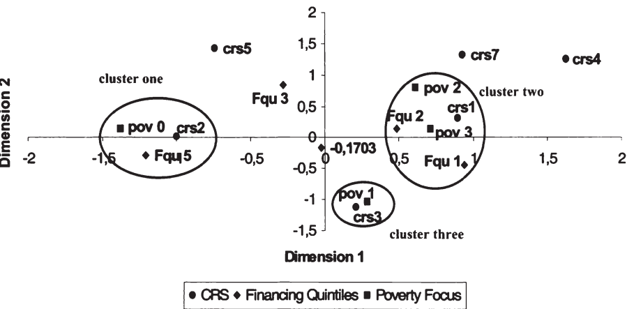
Figure 21: Correspondence Analysis: poverty focus (pov), crs and fin_quint (Fqu)
