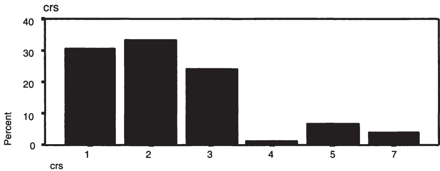
Figure 18: Histogram by Financial Costs
