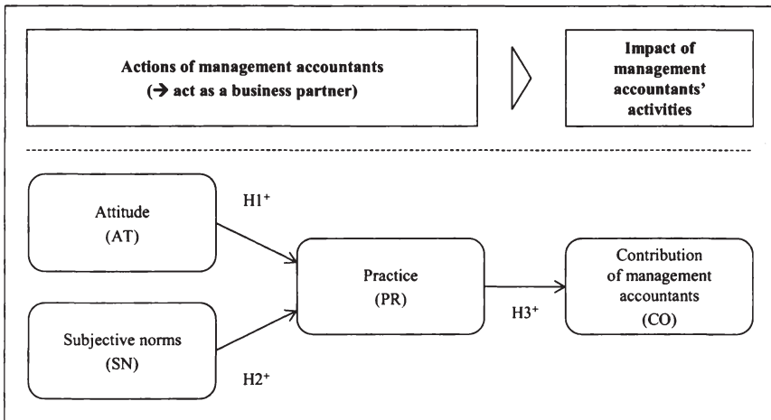
Figure C-2: Research model
