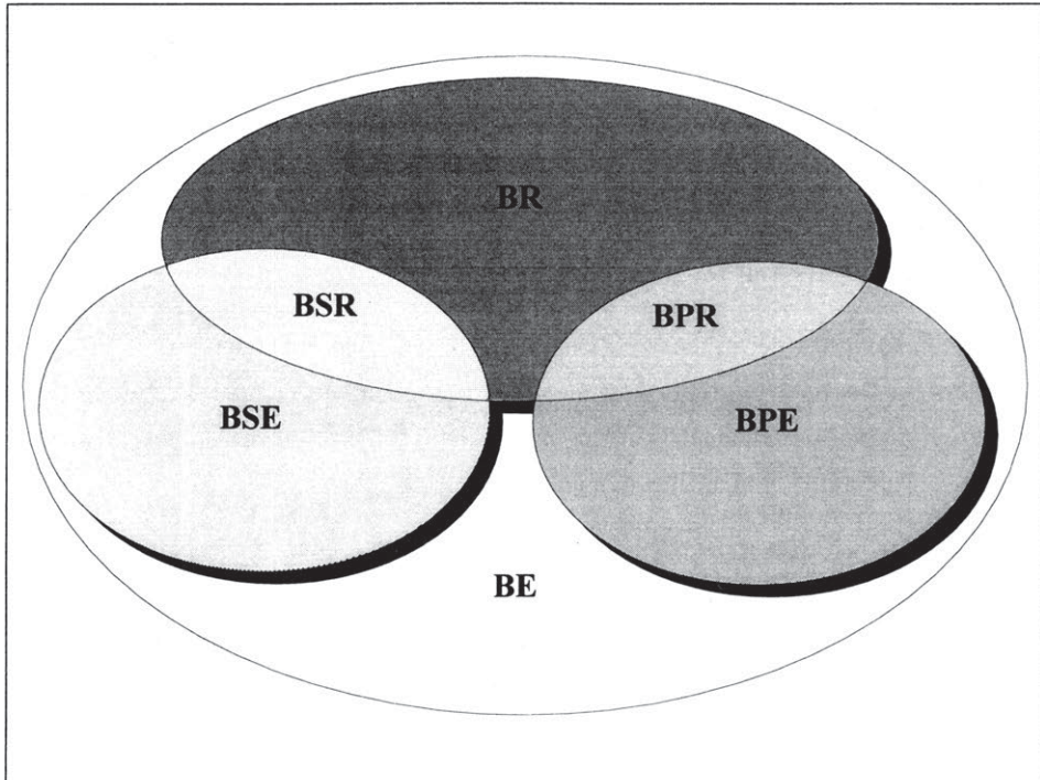
Abbildung 5-5: Business Engineering.
