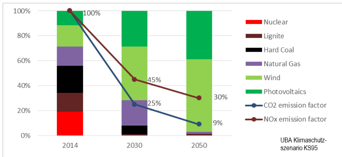
Figure 1: Energy by fuels, Germany, KS95 scenario
